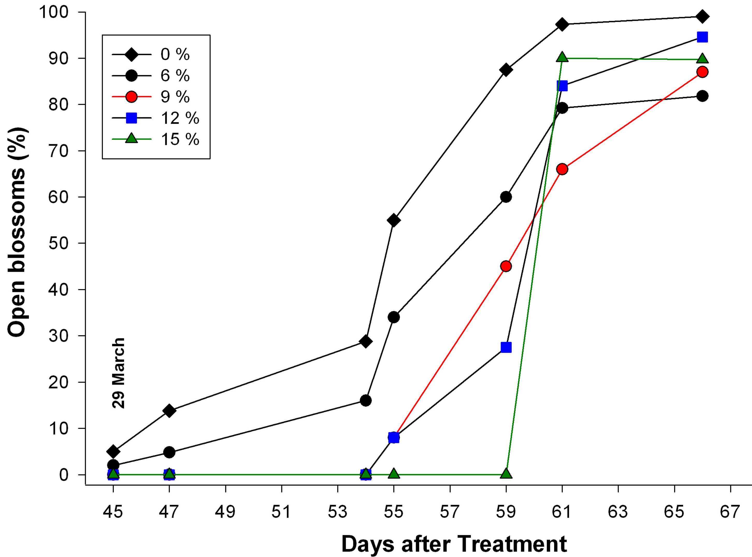
Figure 2. Effect of soybean oil concentration on delay of bloom of 'Legend' blueberry at Spring Hill, Tennessee, 2004.
