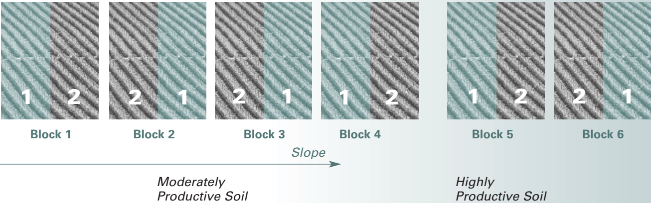
Figure 2. Replicated and randomized side-by-side experiment
