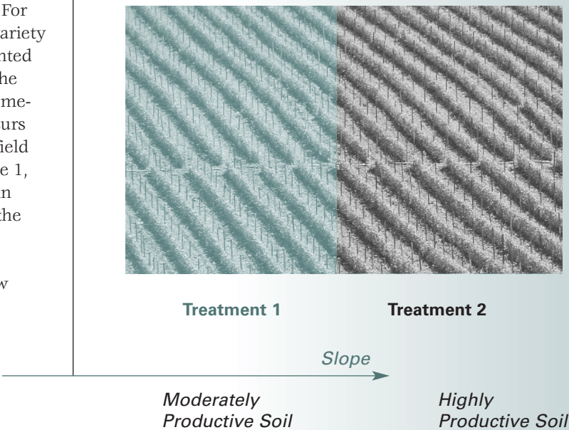
Figure 1. Side-by-side observational experiment.
